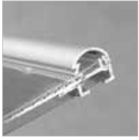
Profile / UYUP007700 0.59" Aluminium Snap profile set (top & bottom) in 118.11" without springs. Top Profile is silver anodized. Bottom profile is mill finished.
